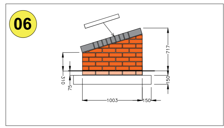
06 Inclined plinth to house memorial plaque. Plinth will be constructed of Red and blue engineering brick and will be constructed to protect the the existing stone plaque.
