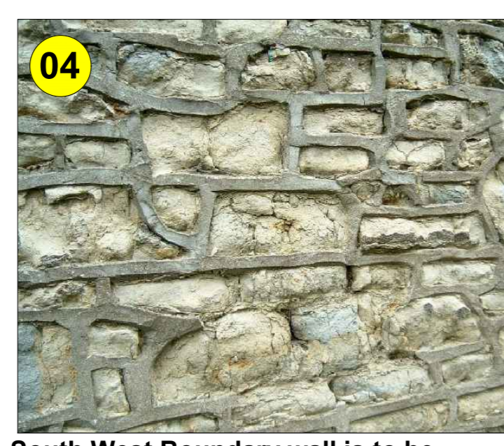
04 South West Boundary wall is to be repointed where necessary. Pointing is to be Ribbon pointing as shown on photograph, in addition sections of the stonewall need to be repaired.
