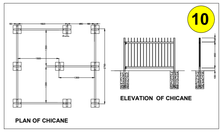
10 Provide and install small Chicane to main entrance to park opposite Church Road.
