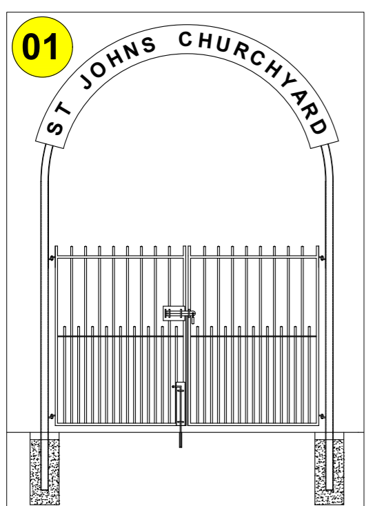
01 Bespoke purpose made service entrance gate with distinctive archway suitable for high sided vehicles. Colour of Unit is to be black to match existing railings.
